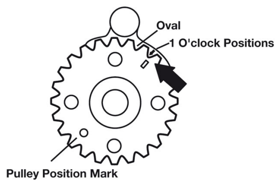
Tool and Crankshaft Pulley with Aligned Timing Mark
